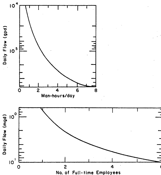
Figure 2-2. Personnel needs for land treatment portion of slow rate systems.
